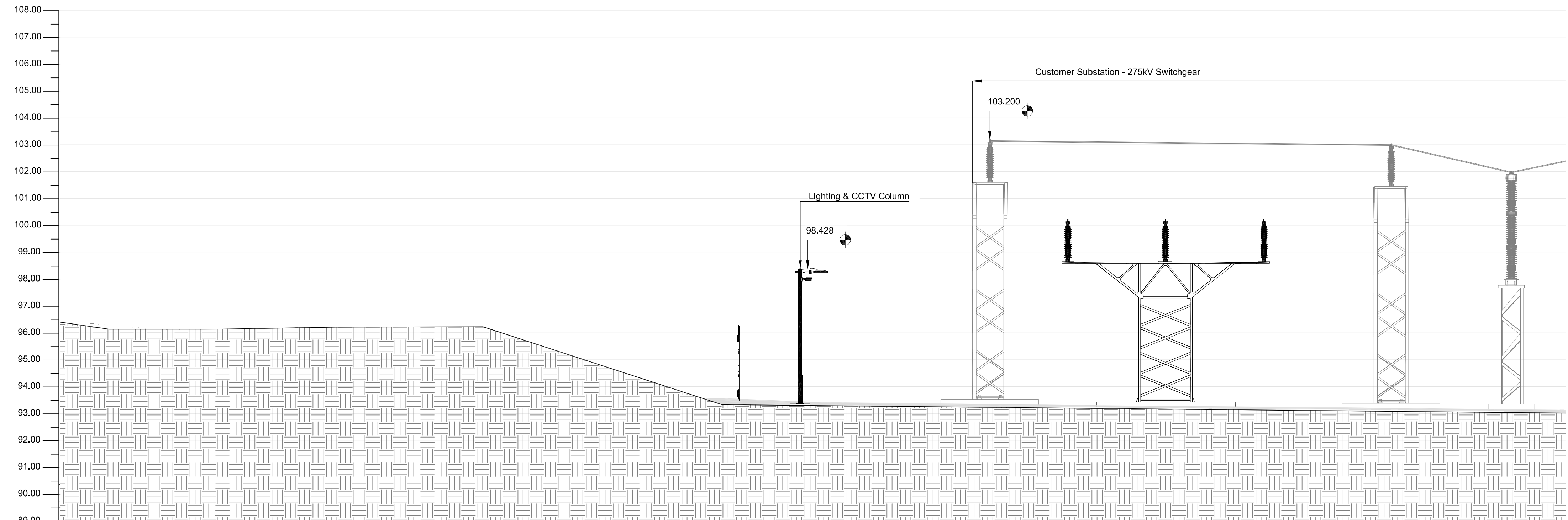
24 SECTION H - H CONTINUED Scale: 1:100
